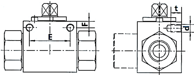
侧面单边螺纹安装孔 (SS)
