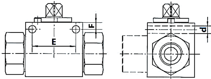
侧面安装通孔 (TH)
